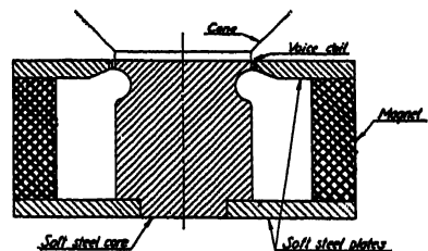
Cross-hatched area indicates the ring-shaped permanent magnet used in one type of permanent-magnet dynamic loudspeaker.
